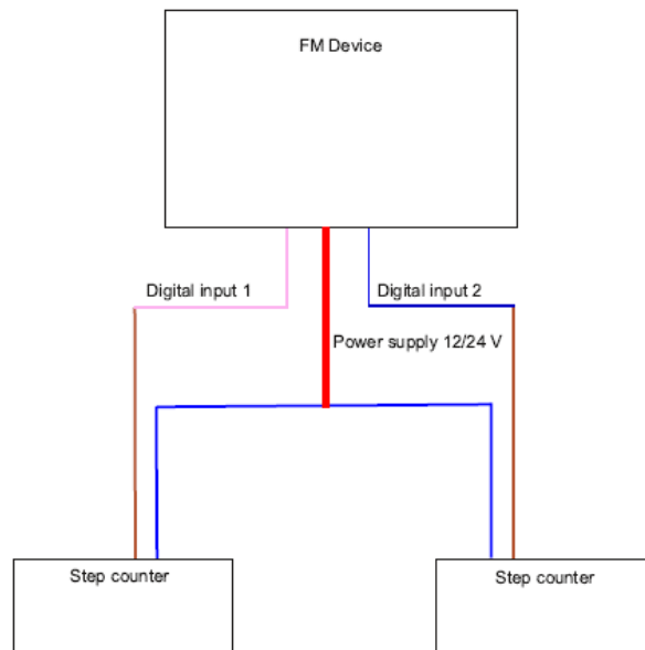
Step detector connection to FM device
